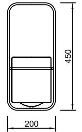
1827 Wall lamp Matt black E27 Max. 10W
